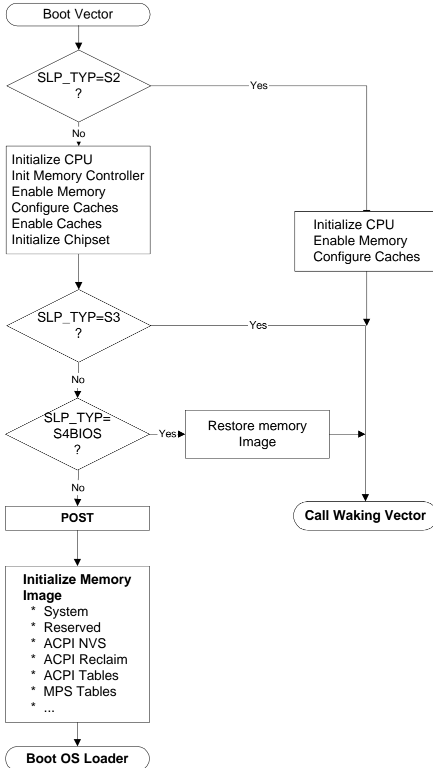
Figure 9-2 BIOS Initialization
