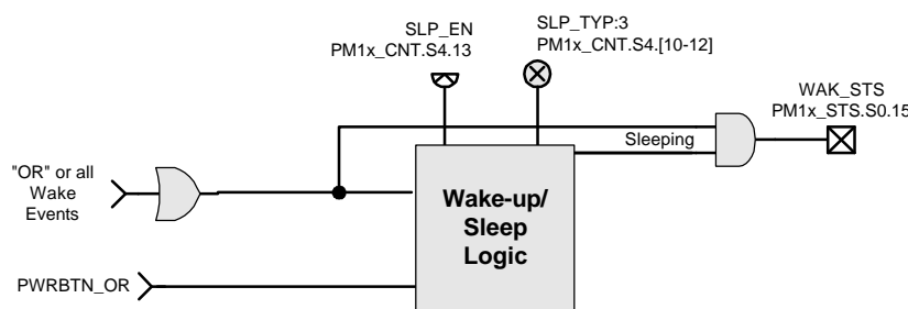
Figure 4-10 Sleeping/Wake Logic
