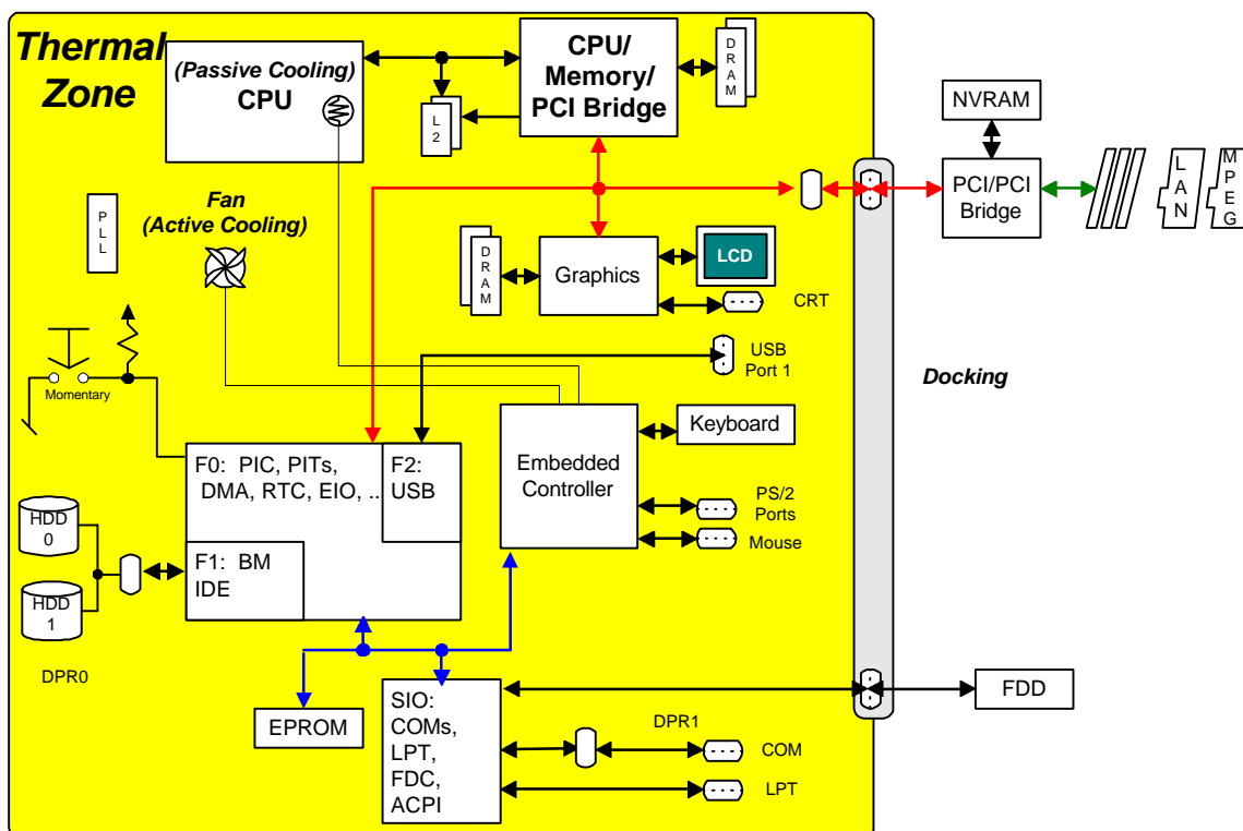
Figure 3-6 Thermal Zone
