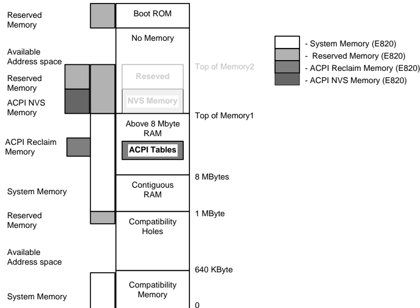
Figure 9-4 Memory as Configured after Boot
