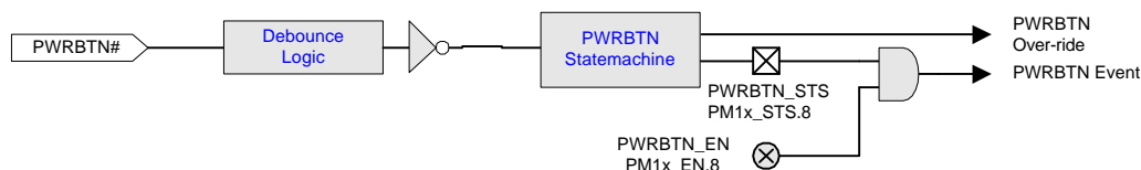
Figure 4-8 Fixed Power Button Logic
