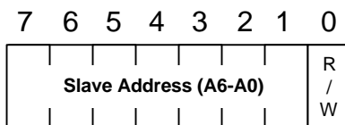
Figure 15-1 SMBus Slave Address Protocol
